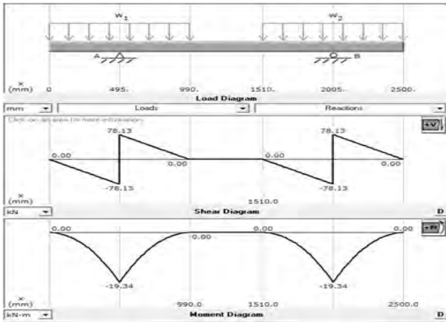
Figure 5 Shear force and bending moment diagrams for zero center binding coefficient
