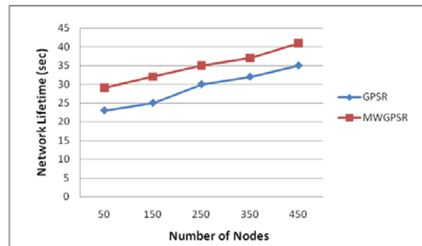
Figure 12 Network Lifetime (15% Node Failure, Speed 15m/s)
