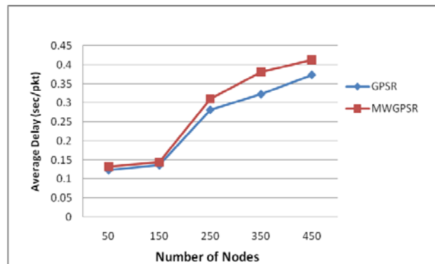
Figure 8 Average Delay (no Node Failure, Speed 10m/s)
