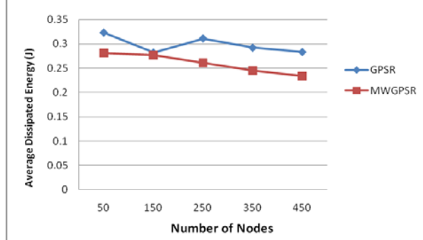
Figure 6 Average Energy Consumption (no Node Failure, Speed 10m/s)
