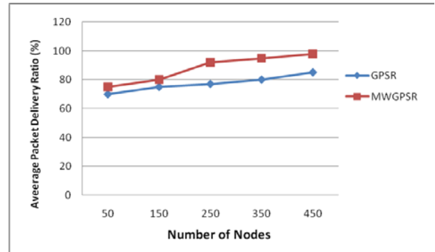
Figure 11 Average Packet Delivery Ratio (15% Node Failure, Speed 15m/s)
