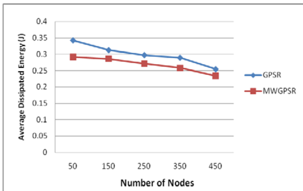
Figure 10 Average Energy Consumption (15% Node Failure, Speed 15m/s)
