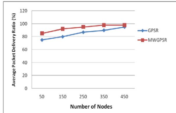
Figure 7 Average Packet Delivery Ratio (no Node Failure, Speed 10m/s)
