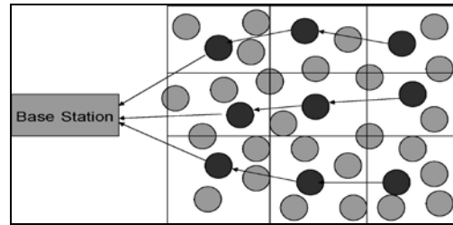
Figure 3 Virtual grid formations in a GAF
