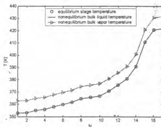
Figure 9 Comparison of temperature profiles resulted from equilibrium and non-equilibrium models.
