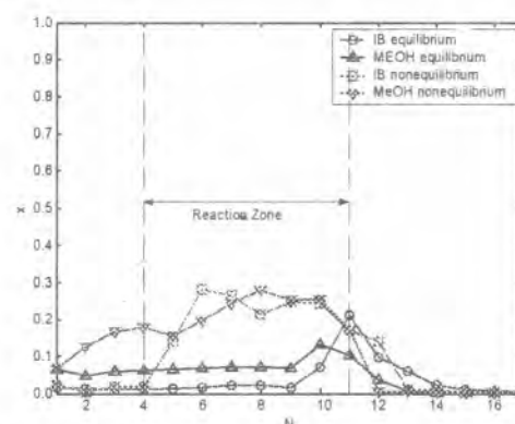
Figure 7 Comparison of concentration profile of reactants for equilibrium and nonequilibrium model simulations for IB and MeOH.
