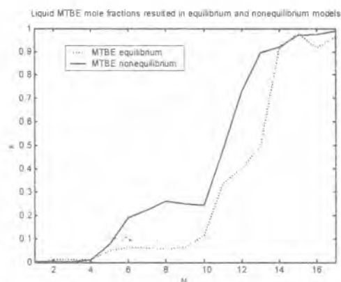
Figure 6 Comparison of concentration profile of MTBE for equilibrium and non-equilibrium model simulations.
