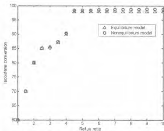
Figure 13 Comparison of isobutene conversion with reflux ratio for equilibrium and nonequilibrium models.
