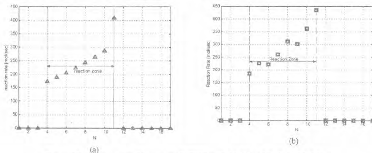
Figure 10 Reaction rate of formation of MTBE with (a) EQ and (b) NEQ Models
