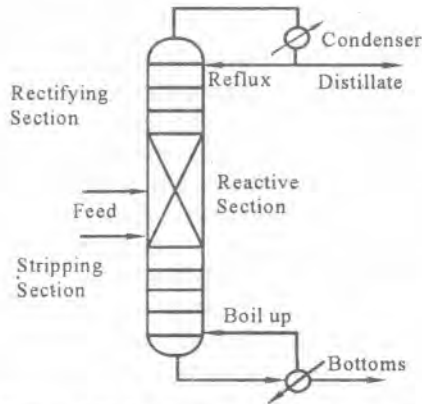
Figure 1 Hybrid reactive distillation column for ether synthesis
