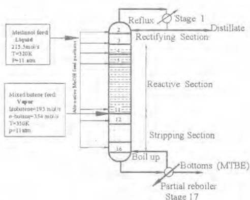
Figure 3 Configuration of the MTBE synthesis column
