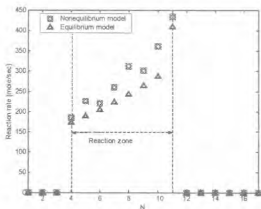
Figure 11 Comparison of reaction rate profiles of formation of MTBE using equilibrium and nonequilibrium models.
