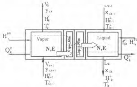
Figure 2 Nonequilibrium stage model for pseudo homogeneous reaction in the liquid phase
