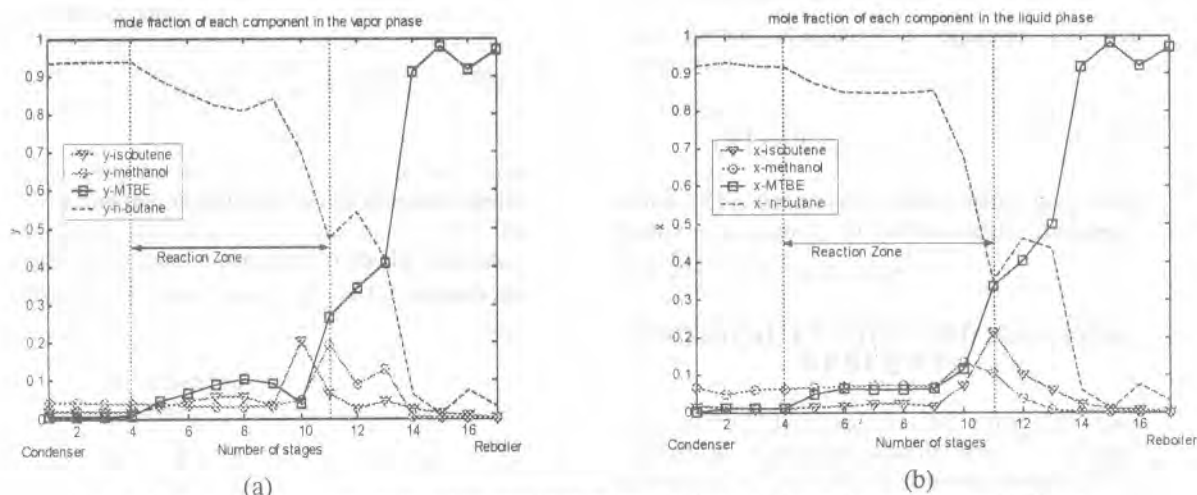
Figure 4 Concentration profiles using equilibrium model for (a) Vapor Phase (b) Liquid Phase
