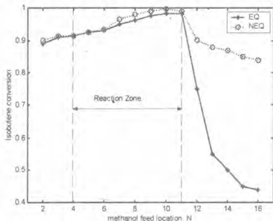
Figure 12 Comparison of Isobutene conversion with methanol feed location with the equilibrium and nonequilibrium models.
