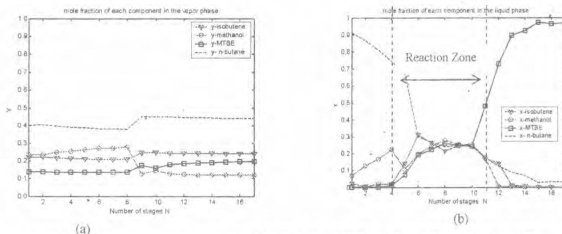
Figure 5 Concentration profiles using nonequilibrium model for (a) Vapor Phase (b) Liquid Phase
