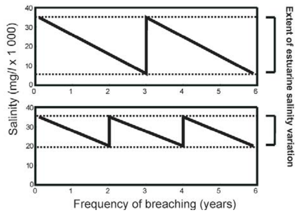
Figure 8 Relationship between breaching frequency and salinity range
