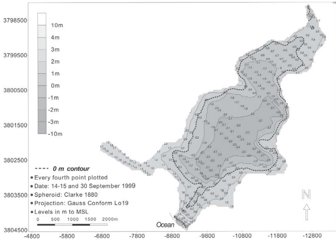
Figure 2 Bathymetry of the Bot River Estuary
