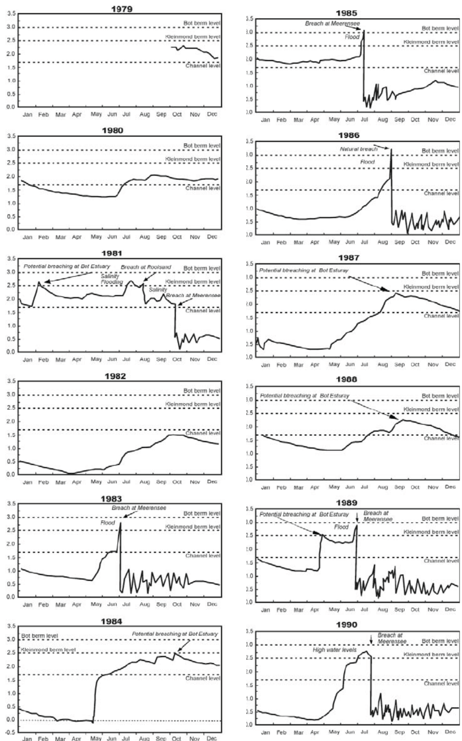
Figure 6 a Bot River Estuary water levels from recorder G4R003 (1979-1990)
