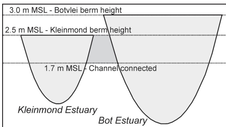
Figure 5 Schematic illustration of the import water levels at which the Bot and Kleinmond Estuaries interact
