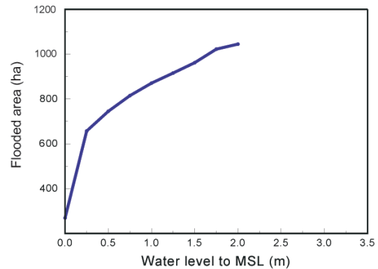
Figure 3 Relationship between water level and area cover increase
