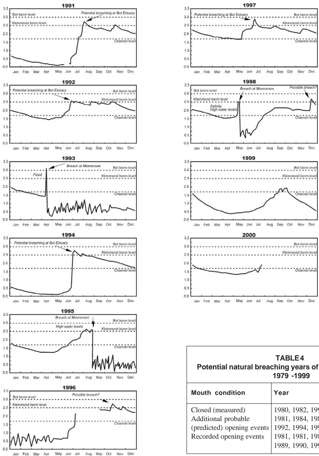
Figure 6 b Bot River Estuary water levels from recorder G4R003 (1991-2000)
