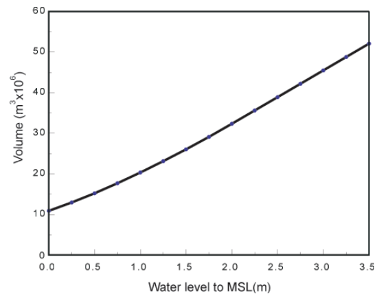
Figure 4 Relationship between water level and volume increase
