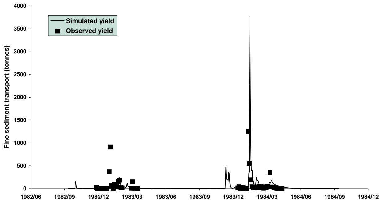
Figure 9 Time series plot of proxy basin validation of simulated sediment transport in the Nyatanda River
