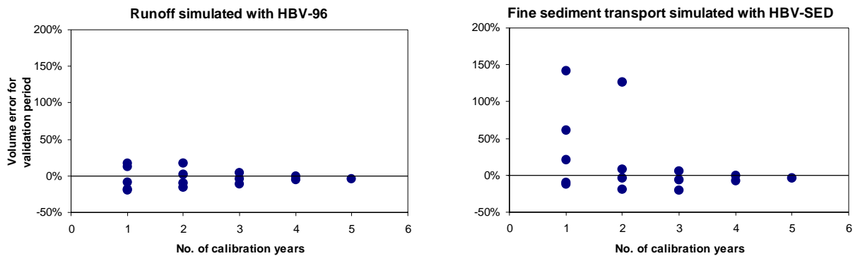
Figure 8 Volume errors for the validation period if different number of years are used for calibration of the HBV-SED model
