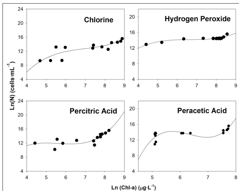
Figure 6. In (Chl-a) vs In(N) plot by fitting the cubic polynomial model with experimental data for M. aeruginosa
