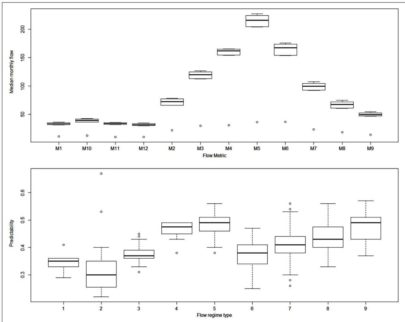
Figure 5. Box-and-whisker plot of median daily flows and 25 th /75 th percentiles for Flow Type 10 for Region 8, Thukela catchment ( n = 8 ; metrics M1-M12 refer to median monthly flows for October–September) (top); and box-and-whisker plot of median and 25 th /75 th percentiles for predictability values across nine flow types for Region 1 (winter rainfall; n = 764 ) (bottom)
