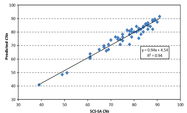
Figure 8 Predicted CN values versus SCS-SA CN values
