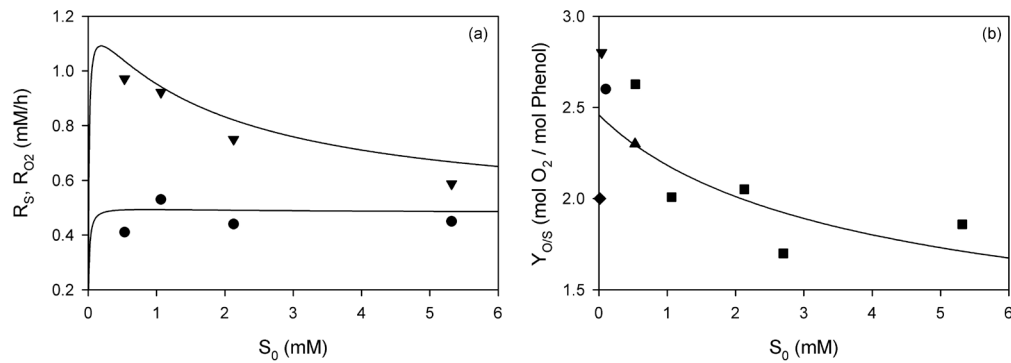
Figure 5 Effect of the initial phenol concentration ( S_0 ) on (a) phenol ( R_S , circles) and oxygen ( R_{O_2} , triangles) consumption rates (a) and on (b) the overall oxidation coefficient ( Y_{O/S} ) measured in this work (squares) and by other authors: Chudoba et al. (1985) ( \blacktriangledown ), Orupold et al. (2001) ( \bullet ), Contreras et al. (2008) ( \blacktriangle ), Lepik and Tenno (2011) ( \blacklozenge ). Solid lines indicate the results obtained by the proposed model using the coefficients shown in Table 1.
