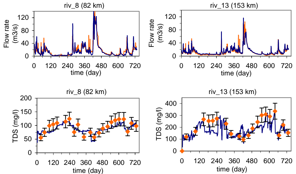
Figure 3 Model calibration: comparison of measured and simulated data sets of TDS concentrations and river flow rate at 82 and 153 km
