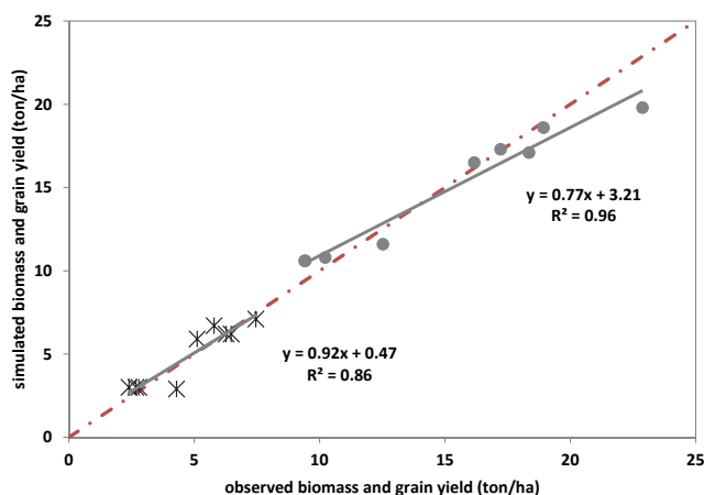
Figure 2 Observed versus simulated final above-ground biomass (dots) and grain yield (stars) for the calibration fields. Continuous lines are the fitted linear trend lines while the dashed line is the one to one (1:1) line for comparison. Linear functions and the respective R^2 (goodness of fit coefficient of determination) values are shown.
