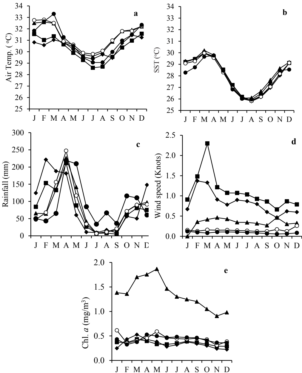
Figure 3. Average a) maximum air temperature, b) sea surface temperature, c) rainfall, d) wind speed and e) chlorophyll a in Mtwara (◆), Lindi (■), Pwani (▲), Dar es Salaam (○) and Tanga (●) during 2004 – 2010.
