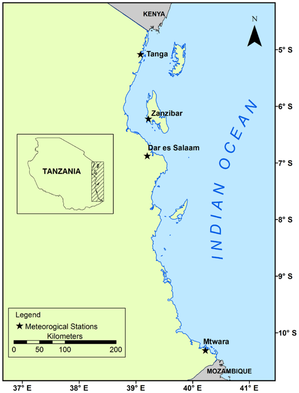
Fig. 1: Map of the coastal Tanzania showing the sites of meteorological stations
