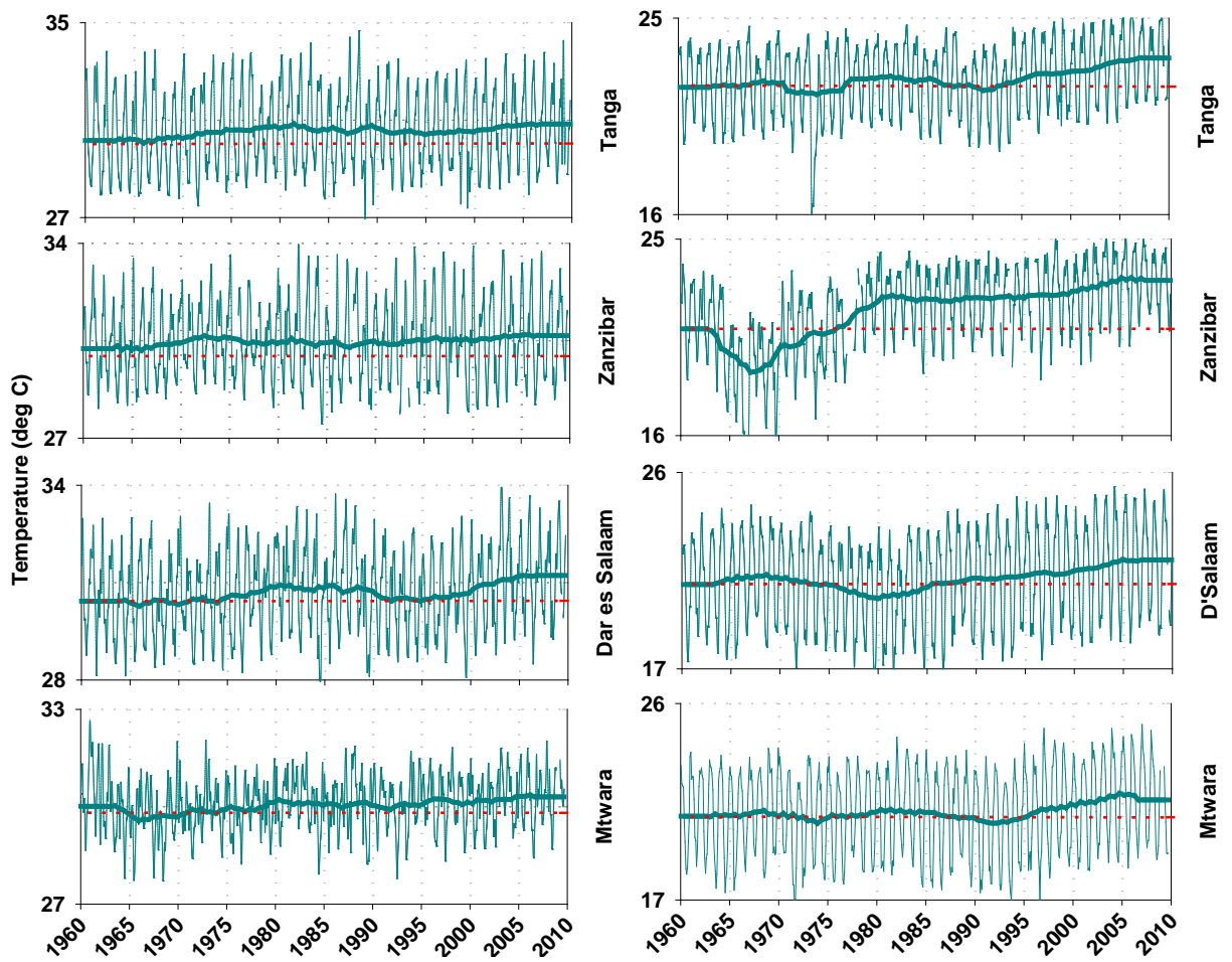
Fig. 2: Monthly variations of maximum (left) and minimum (right) temperatures at the four study sites. The bold lines represent the Loess fit and the red dashed line corresponds to the average level in 1960.
