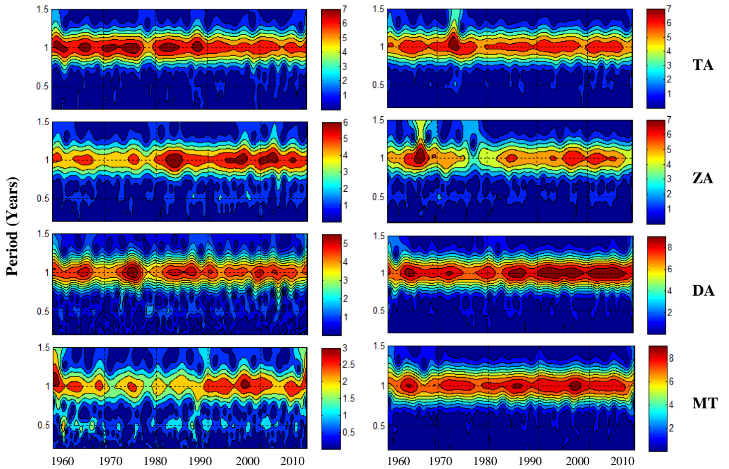
Fig. 3: Wavelet spectra depicting the annual cycle of maximum temperatures (left panel) and minimum temperatures (right panel) at Tanga (TA), Zanzibar (ZA), Dar es Salaam (DA) and Mtwara (MT). The legend on the right represents temperature ( ^{\circ}\text{C} )
