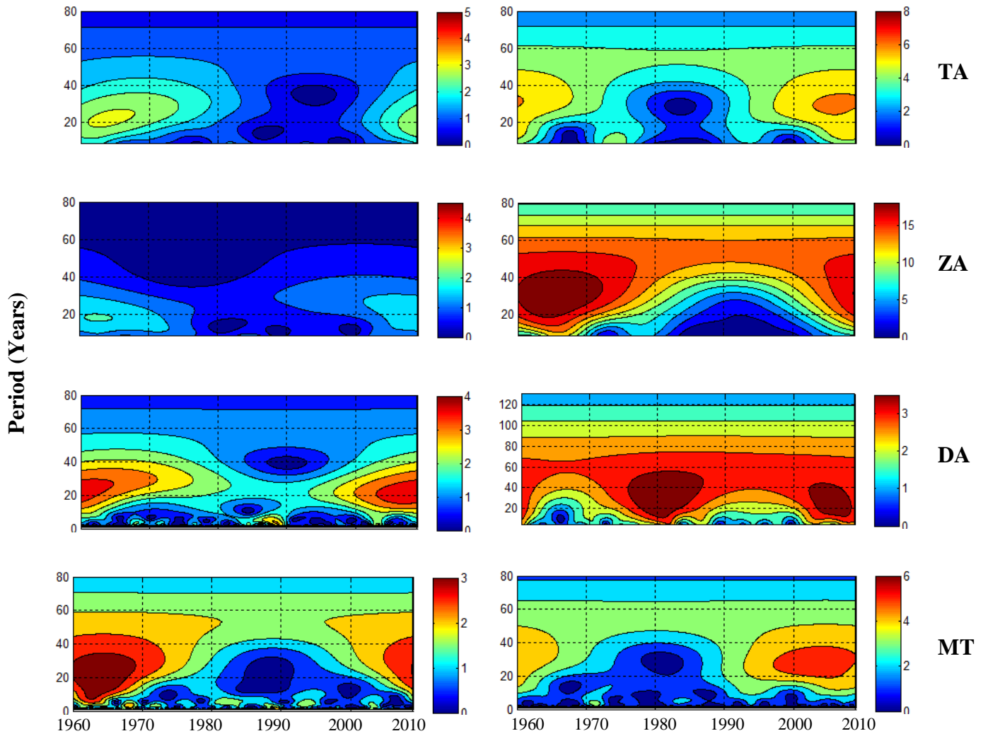
Fig. 4: Same as in Fig. 3 above, but for the low frequency inter-decadal oscillations.
