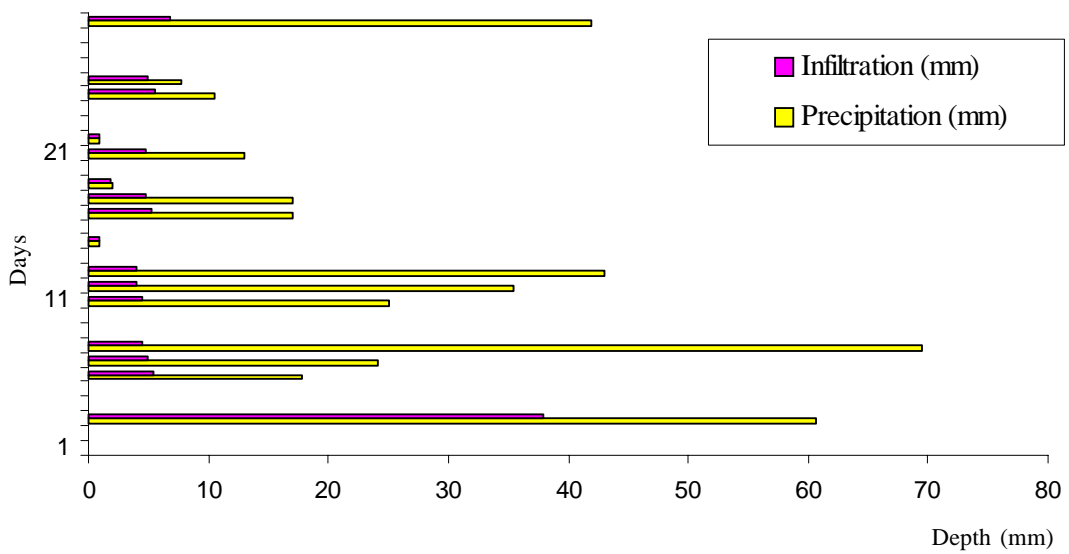
Fig. 3. Comparison of precipitation with infiltration in September
