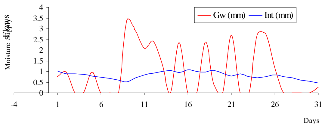
Fig. 6. Groundwater and interflow variation in October
