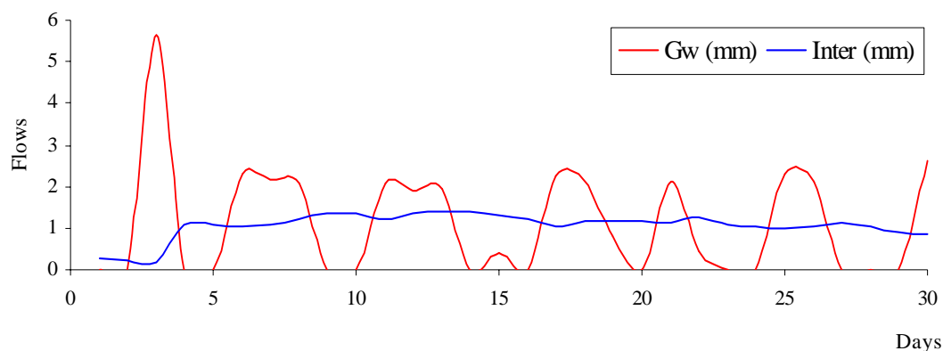
Fig. 5. Groundwater and interflow variation in September
