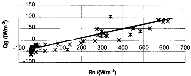
Fig. 6. Qg-Rn relations for April 1996.
