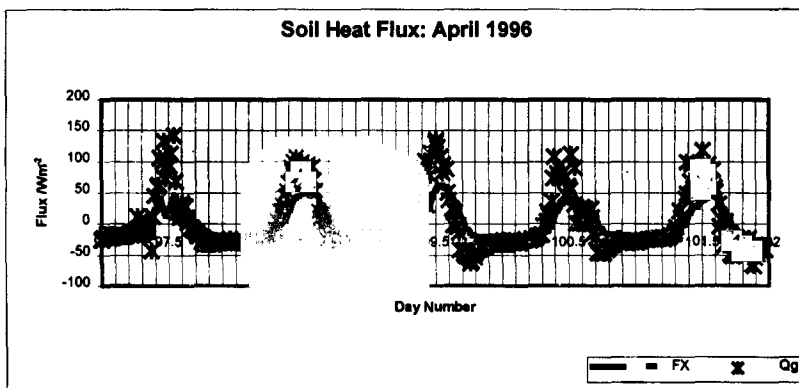
Fig. 3. Soil Heat Flux
