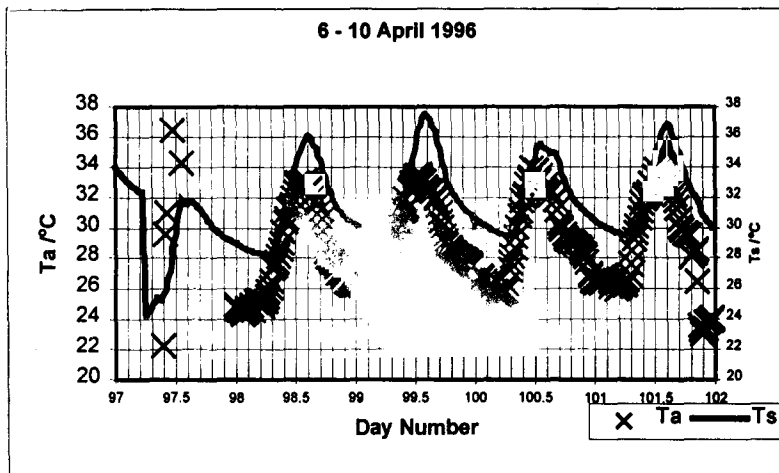
Fig. 2. Air and soil temperatures
