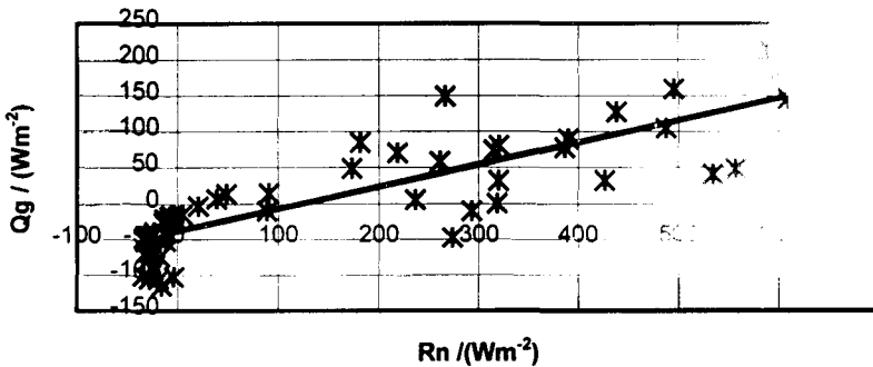
Fig. 4. Qg-Rn relations for October 1994.
