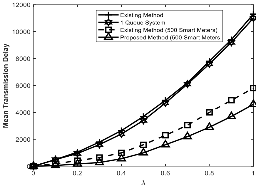
Figure 11: Mean transmission delay vs packet generation.
