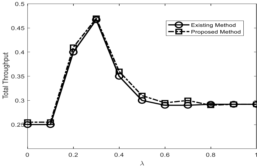
Figure 9: Variation of throughput with packet generation rate.
