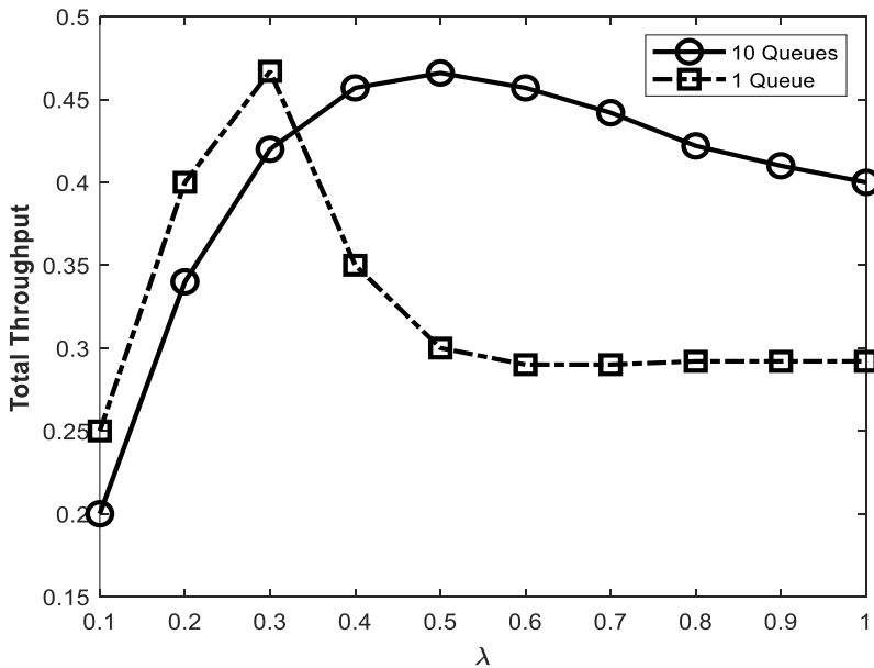
Figure 8: Variation of throughput with packet generation rate.
