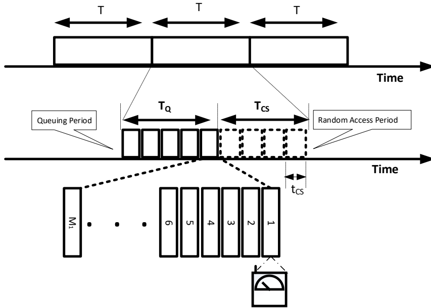
Figure 4: Queuing and random-access timing.
