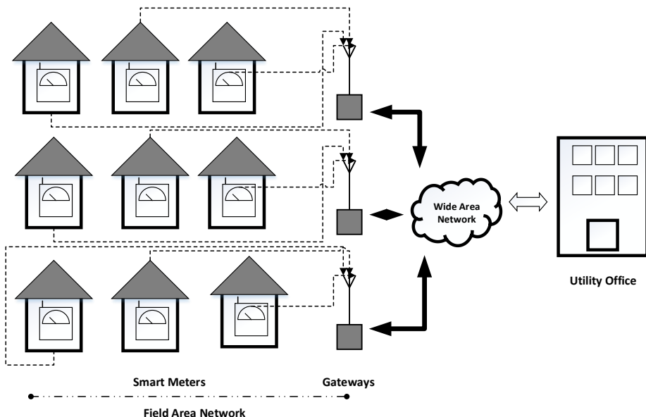
Figure 1: AMI architecture.
