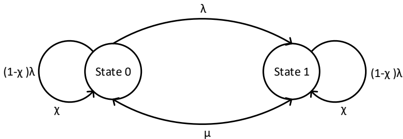
Figure 5: Transition state diagram.
