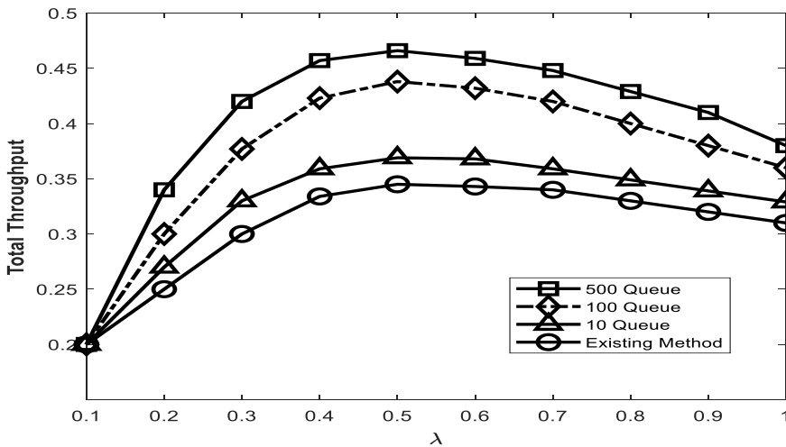
Figure 10: Total throughput with packet generation at different queue sizes.
