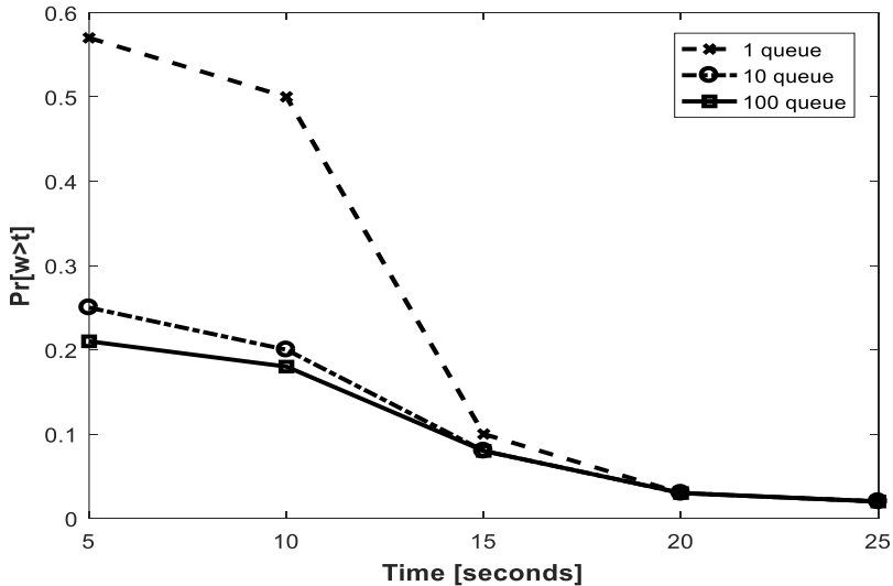
Figure 6: Variation of delay tail probability with time.
