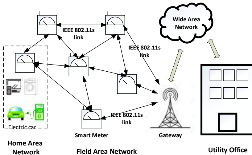
Figure 2: IEEE 802.11s based AMI architecture.
