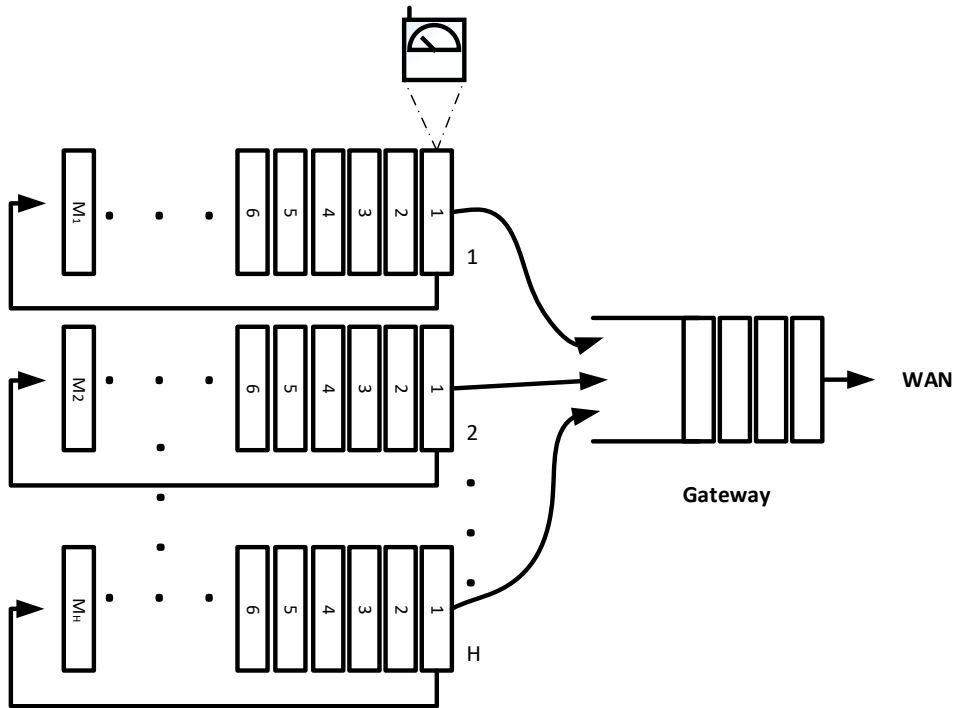
Figure 3: Proposed logical AMI model.
