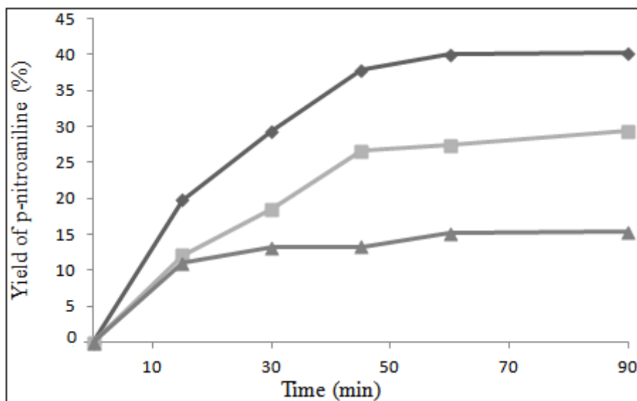
Figure 7: BAPNA hydrolysis catalyzed by trypsin enzymes; \blacklozenge free trypsin, \blacksquare trypsin immobilized on SH-CO-MTS, \blacktriangle Trypsin immobilized on SH-DDA-MTS.
