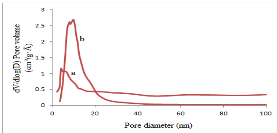
Figure 3: Pore size distribution of SH-CO-MTS (a) and CO-MTS (b).
