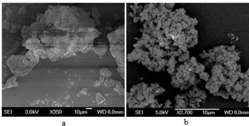
Figure 5: SEM images of CO-MTS (a) and SH-CO-MTS (b).
