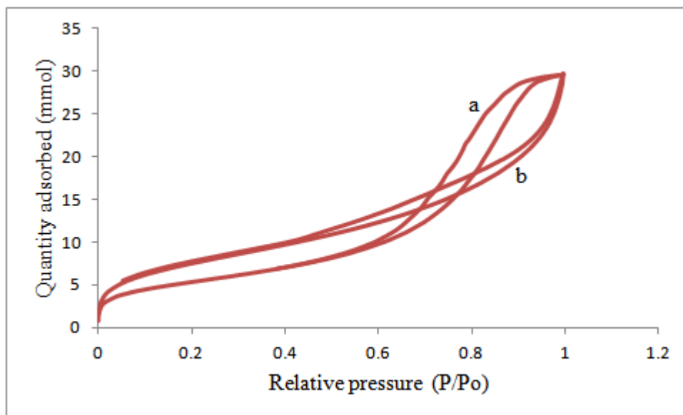
Figure 2: Nitrogen adsorption-desorption isotherms for (a) CO-MTS and (b) SH-CO-MTS.
