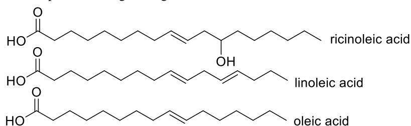
Figure 1: Major components of castor oil fatty acids.
