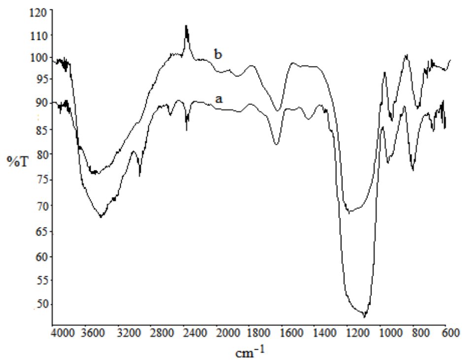
Figure 4: FTIR spectra for SH-CO-MTS (a) and CO-MTS (b).
