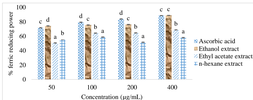
Figure 2: Percentage ferric reducing powers of the ethanol, ethyl acetate and n-hexane extracts of M. indica leaves. Values are presented as mean \pm standard deviation of triplicates. Values with different superscripts at the same concentration are significantly different at p < 0.05 .
