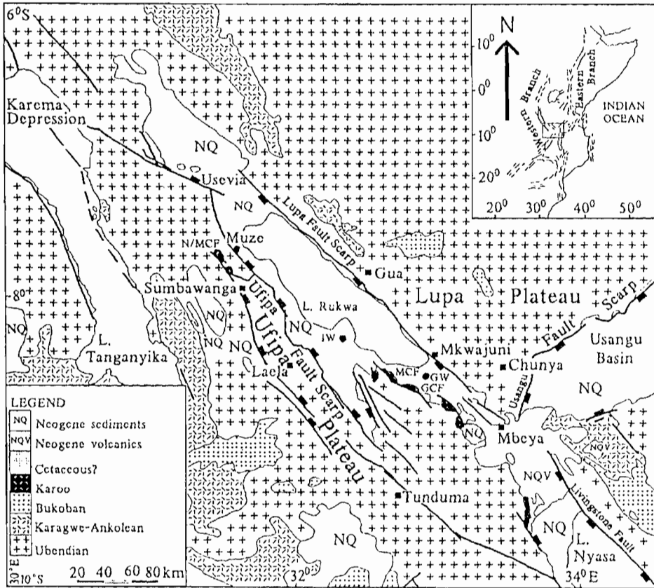
Fig. 1: The Geological Map of South-Western Tanzania showing the location of study area: IW = Ivuna Well; GW = Galula Well; GCF = Galula Coal-Field; MCF = Muasa Coal-Filed; N/MCF = Namwele/Mkomola Coal Field
