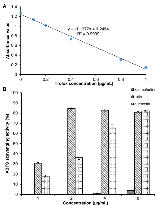
Figure 6: Antioxidant effect of kaempferitrin on ABTS radicals
