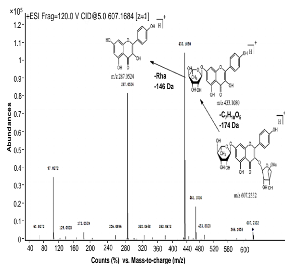
Figure 4: The mMass fragmentation pathway of component 3
