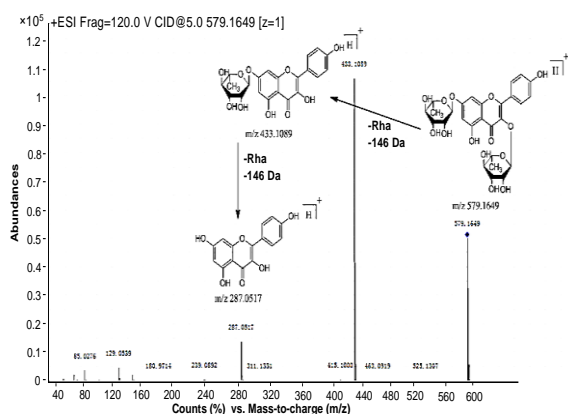
Figure 2: The mass fragmentation pathway of component 1
