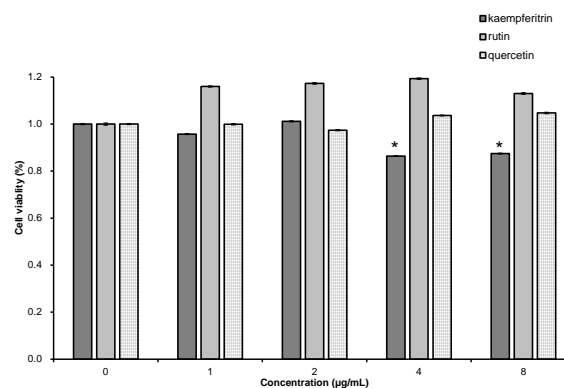
Figure 7: Anti-proliferation activity of kaempferitrin on SMMC-7721 cells in vitro
