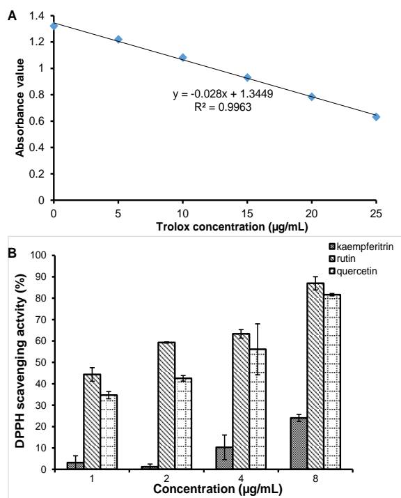
Figure 5: Antioxidant effect of kaempferitrin on DPPH radicals
