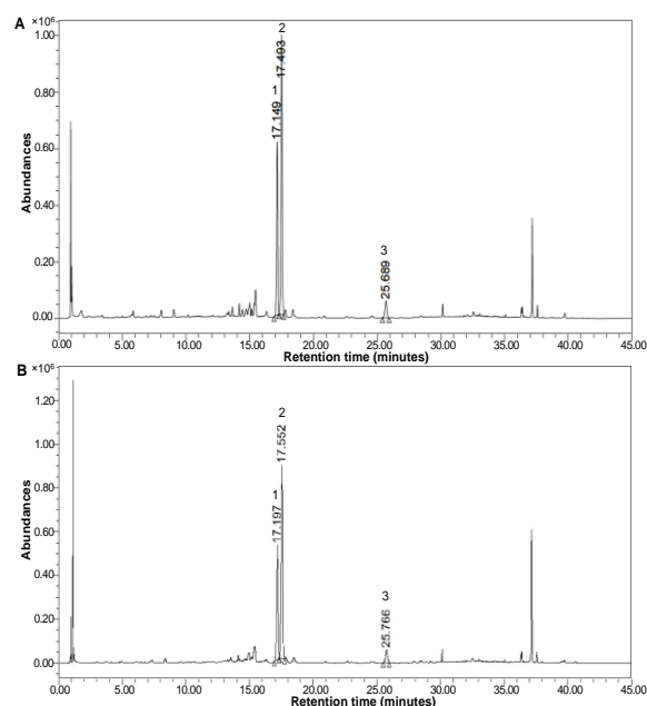
Figure 1: The UPLC spectra of C. ambrosioides at 265 nm UV. A: 80 % methanol; B: 80 % ethanol
