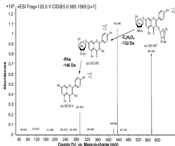
Figure 3: The mass fragmentation pathway of component 2
