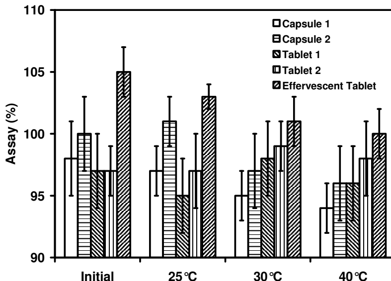
Figure 3: Initial assay results for the sennoside products compared to the assay results after being stored for 12 weeks at 25°C + 60 % RH; 30°C + 60 % RH; 40°C + 75 % RH
