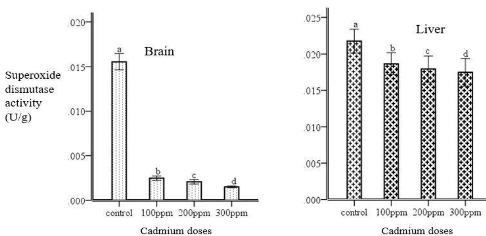
Figure 2: Effects of cadmium on brain and liver superoxide dismutase (SOD) activity. Each bar represents the mean ± SEM (n = 8); bars with different alphabets are significantly different at p < 0.05
