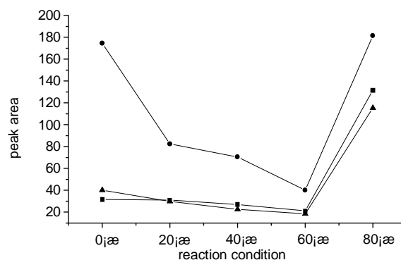
Figure 2: Analysis of CA enzymatic oxidation in mimic system II. Note: ■ = peak 2; ● = peak 5 (CA); ▲ = peak 7
