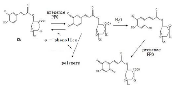
Figure 4: CA oxidation pathway in the mimic enzymatic oxidation system
