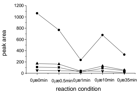
Figure 1: Analysis of CA enzymatic oxidation in the mimic system I. Key: ■ = peak 2; ● = peak 5 (CA); ▲ = peak 7; ▼ = peak 8
