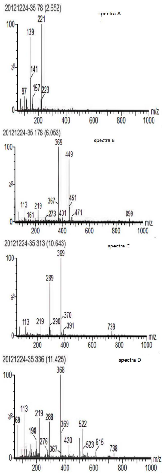
Figure 3: ESI mass spectra of enzymatic oxidation products of CA. From spectra A to D: peak 2, peak 8, peak 22, and peak 23
