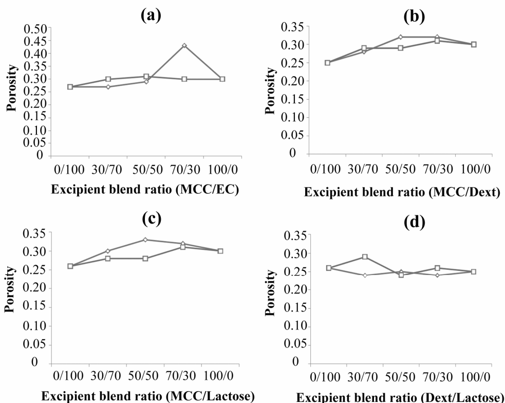
Fig 3: Effect of excipient mixture ratio on the porosity of binary (◆) and bilayer (□) tablets compressed at 61.9 MPa
