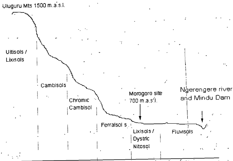
Figure 2 (b): A catena from Uluguru Mts. to Ngerengere river. (Modified from Moberg et al. , 1982; with data from Kaaya, 1989).
