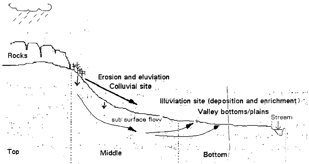
Figure 1: Water moyement in a generalised catena
