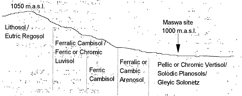
Figure 2(c): A catena across Shishiyu Maswa (constructed with information from Meertens et al. , (1999), Mahoo et al. , (1998), Ngailo et al. (1994) and, De Pauw (1984)
