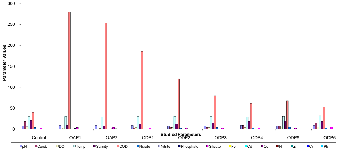
FIG. 4. CONCENTRATION PATTERN OF THE STUDIED PARAMETERS ALONG OWORONSOKI SAMPLE POINTS
