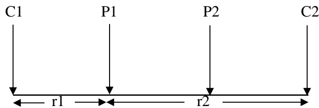
FIG. 3 ELECTRODES CONFIGURATION
