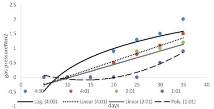
Figure 2: A graph of pressure monitored at different days for different preparations for poultry wastes
