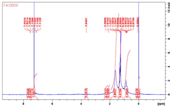
Figure 3: Proton- NMR Spectra of Purified Fraction of Ethylacetate Extract of Acalypha wilkesiana Leaves
