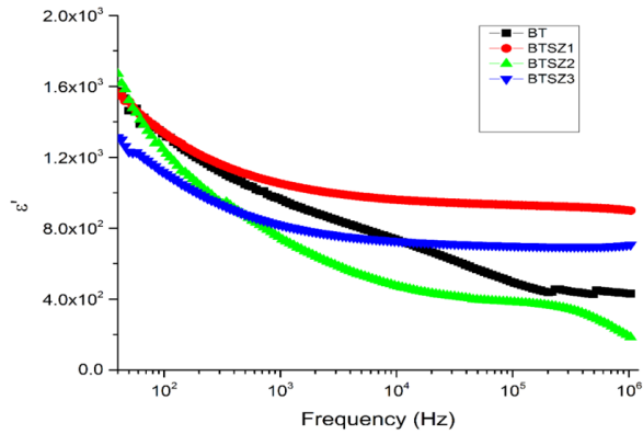
Fig. 4: Variation of real part of relative permittivity ( \epsilon' ) of nanocrystalline BT, BTSZ1, BTSZ2 and BTSZ3 ceramics at 30°C.
