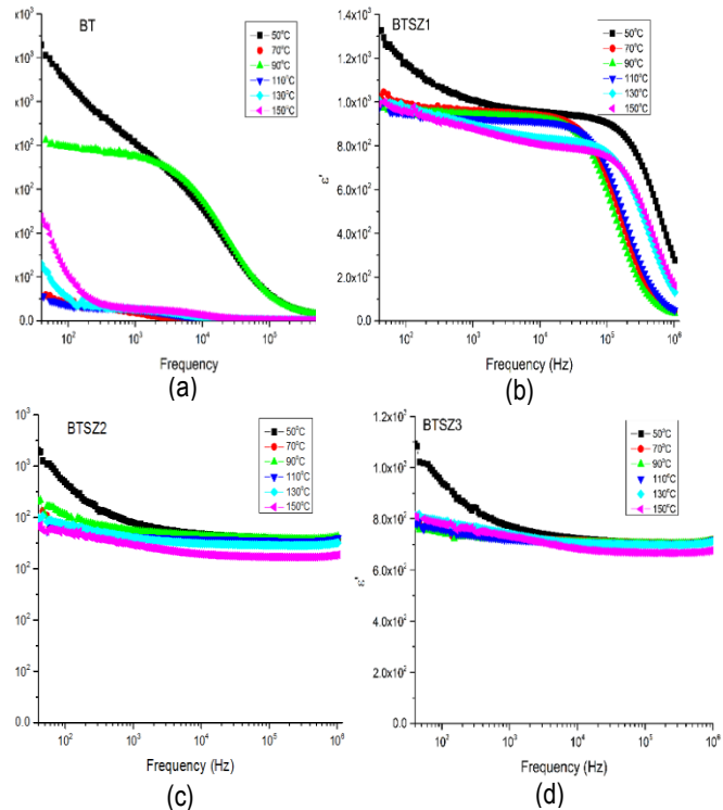
Fig.6 Frequency dependences of real part of relative permittivity nanocrystalline ceramic at various temperature: (a) BT, (b) BTSZ1, (c).BTSZ2 and (d). BTSZ3
