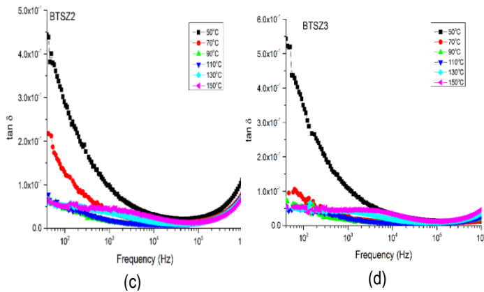
Fig. 7: Frequency dependences of dielectric loss of nanocrystalline ceramic at various temperature: (a). BT, (b) BTSZ1, (c) BTSZ2 and (d) BTSZ3
