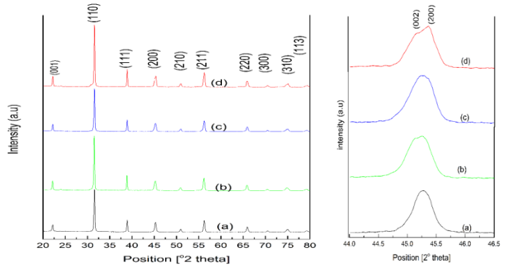
Fig. 2: XRD Patterns of (a). BT (b). BTSZ1 (c). BTSZ2 and (d). BTSZ3 sintered at 1190°C
