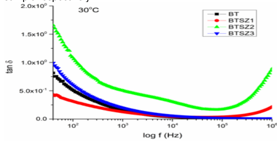
Fig. 5: Variation of loss tangent with frequency of nanocrystalline BT, BTSZ1, BTSZ2 and BTSZ3 ceramics at 30°C.
