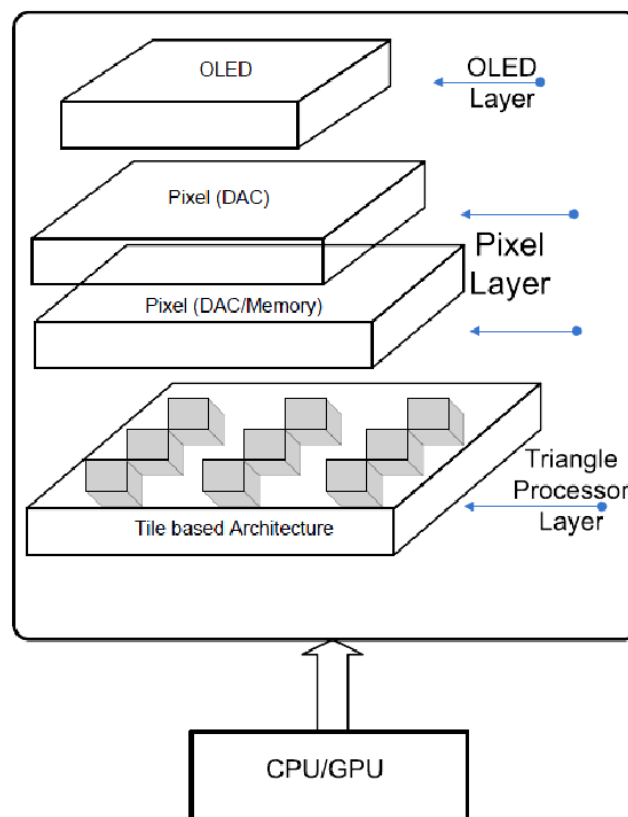
Figure 6: 3D view of Tile based Triangle Processing.
