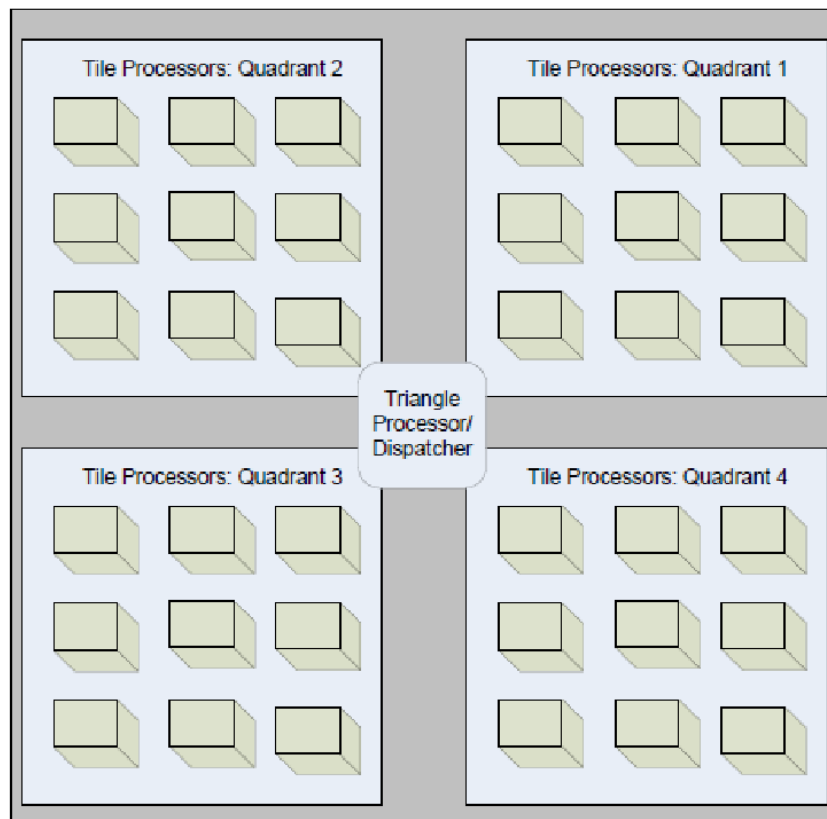
Figure 7: Tile based Architecture for Smart-Display.
