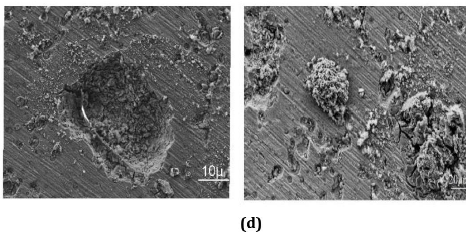
Figure 3. Potentiostatic polarization curves of Al-Zn-In : (a) passive state of the Al-Zn-In andoe SEM observation, (b) Potentiostatic polarization curves of Al-Zn-In at 1050 mV/ECS at (E_{corr} < E_{imp} < E_R) , (c) Potentiostatic polarization curves of Al-Zn-In at 1050 mV/ECS at (E_{imp} > E_R) , d) Active state of the Al-Zn-In andoe SEM observatrin.
