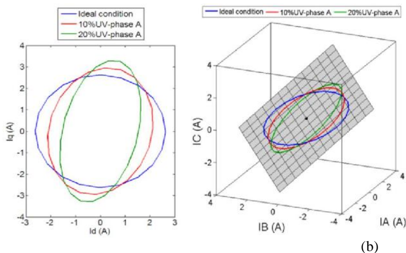
Figure.10 : (a) Current Park's vector patterns; (b) 3D stator current patterns for: 10% and 20% under voltage in phase A
