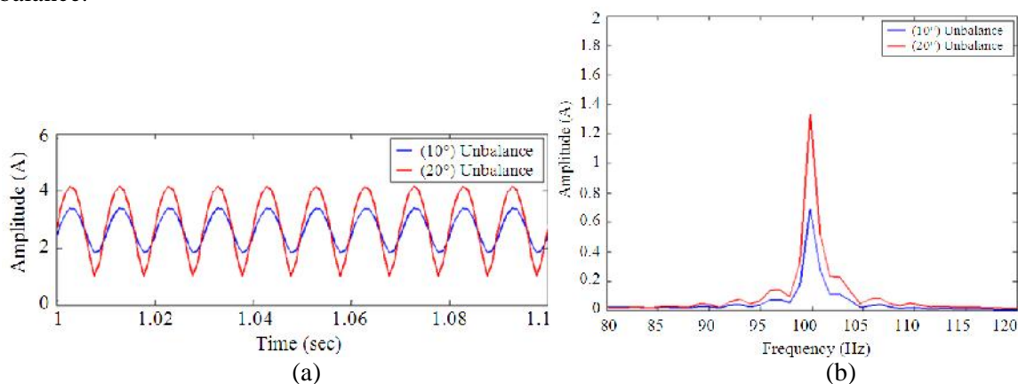
Figure. 17. (a) The motor current Park’s vector modulus; (b) spectrum of the vector Park modulus around the (100 Hz) in case of 10^\circ and 20^\circ angle displacement
