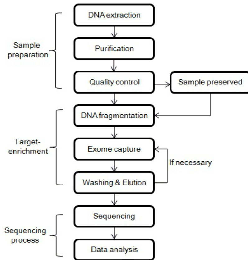
Figure 3: General workflow of exome sequencing [56].
