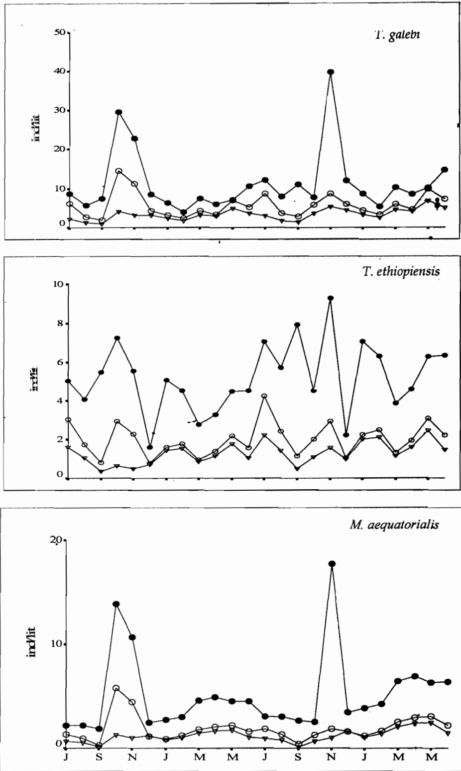
Fig. 3. Numerical density of nauplii(●), copepodites (○ ) and adults (▽ ) for each species of copepoda ( T. galebi , T. ethiopiensis , and M. aequatorialis ) in Lake Tana for the period July 2003 to June 2005.
