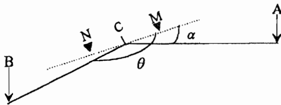
Fig. 5. Imperfect Schlumberger array.
