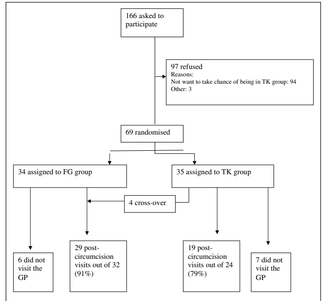
Fig. 2. Trial profile.
