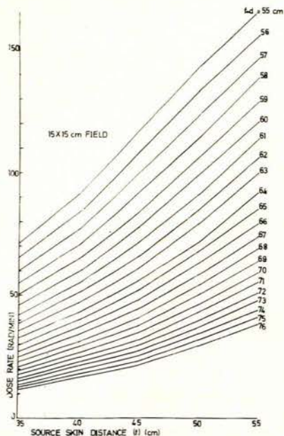
Fig. 5. Variation of central axis depth-dose data with source-skin distance.
