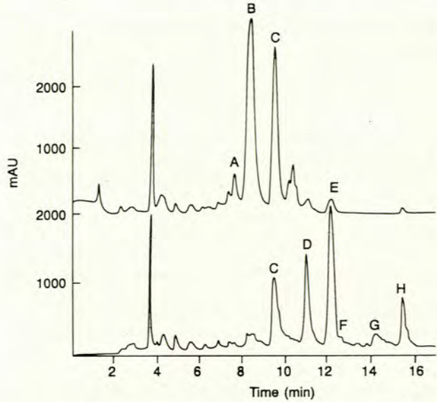
Fig. 8. HPLC chromatogram of human urinary rooperol metabolites 72 hours after incubation without exogenous beta-glucuronidase (upper chromatogram) and with 100 µg/ml exogenous beta-glucuronidase (lower chromatogram). Major changes are the disappearance of peaks A and B and a 50% decrease in peak C and the increase of peaks at retention times (RTs) 11,0 min (D) and 12,1 min (E) which have been shown to be monosulphates of rooperol. 4 Rooperol (RT = 12,6 min, peak F) is a minor peak while dehydroxyrooperol (RT = 14,1 min, peak G) and bis-dehydroxyrooperol (RT = 15,4 min, peak H) are present as described. 4
