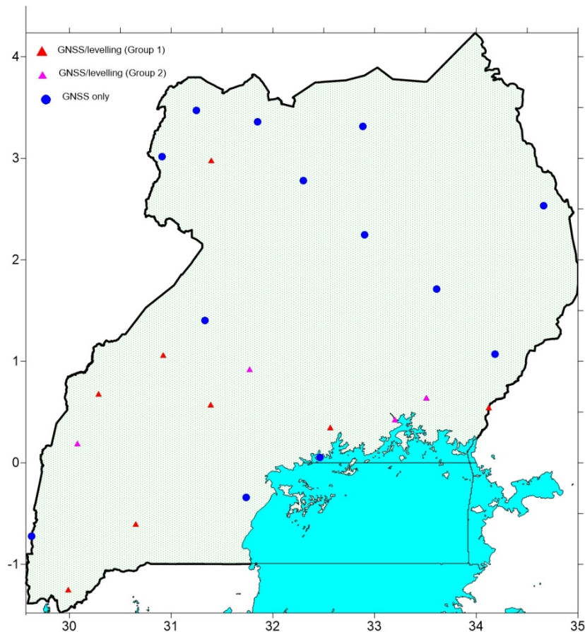
Figure 2: Network of GNSS/levelling and GNSS only points used for the generation of the corrective surface
