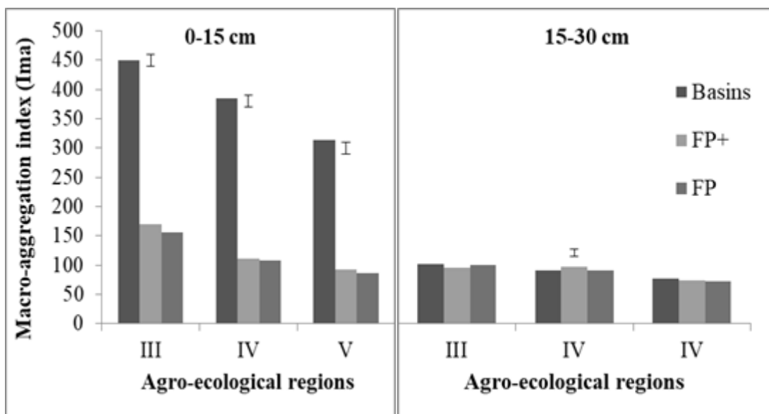
Figure 3: Soil macro-aggregation for two soil depths after three seasons of planting basins (Basins), hand hoeing farmer practice with same fertility amendments as in basins (FP+) and hand hoeing farmer practice without fertility amendments (FP). (Bars represent LSD at P < 0.05 ).
