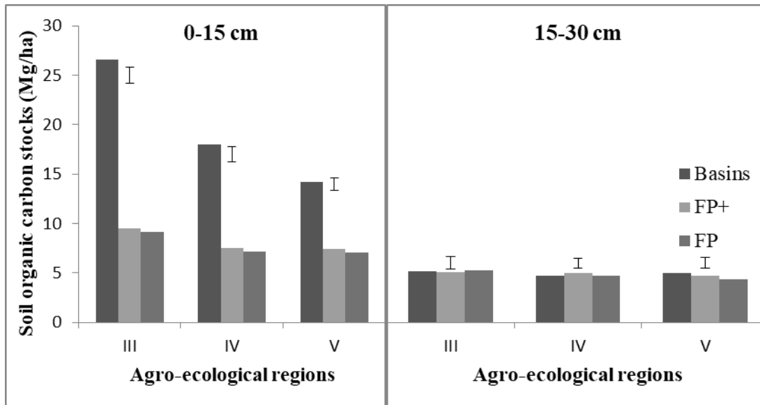
Figure 2: Soil organic carbon stocks (Mg/ha) for two soil depths after three seasons of planting basins (Basins), hand hoeing farmer practice with same fertility amendments as in basins (FP+) and hand hoeing farmer practice without fertility amendments (FP). (Bars represent LSD at P < 0.05 ).
