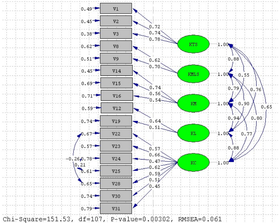
Figure 2 The five factor model – the first order CFA and the standardised solutions. KTS: knowledge of teaching strategies, KMLS: knowledge of mathematical language and symbols, KM: knowledge of misconceptions, KL: knowledge of learners, KC: knowledge of curriculum.
