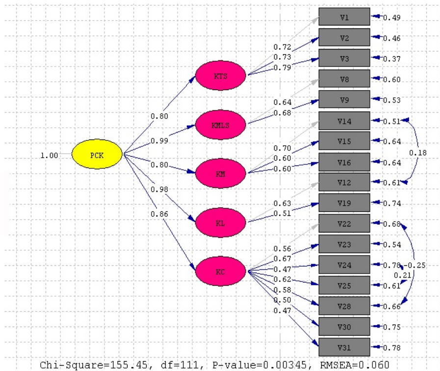
Figure 3 The diagram generated for the second order confirmatory factor analysis and the standardised solutions
