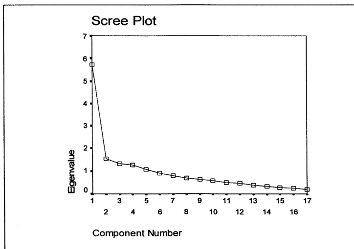
Figure 1 The scree plot analysis result
