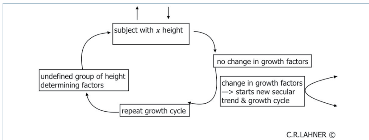
Figure 1: Flow diagram illustrating secular change within a population
