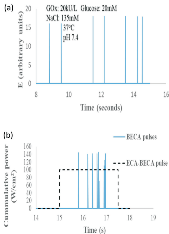
Figure 2 (a) BECA pulses optimized for 20 kU L -1 GOx at pH 7.4 and 37 °C (b) Modelled proposed combined ECA-BECA sustained pulses compared to the high-frequency \mu s and ns BECA pulses
