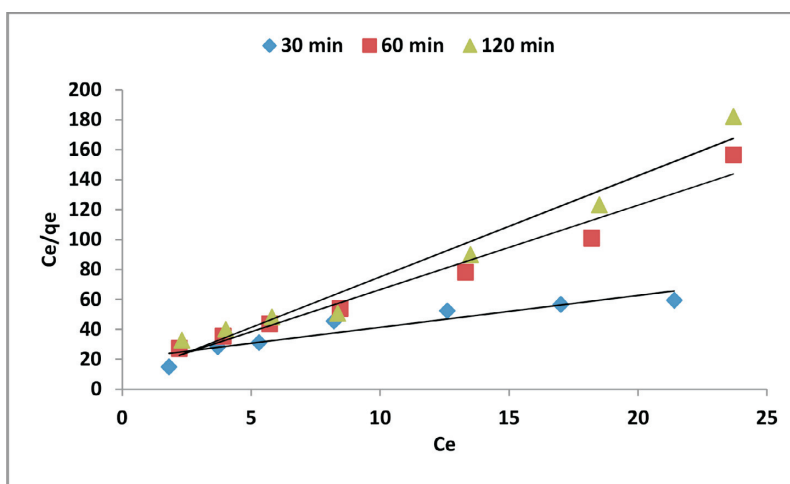
Figure 8 Langmuir isotherm plot for fluoride removal onto \text{Mn}^{2+} incorporated bentonite clay at 30, 60 and 120 min contact time (250 rpm shaking speed, \text{pH } 5.54 \pm 0.5 and adsorbent dosage of 1 \text{ g } 100 \text{ mL}^{-1} ).
