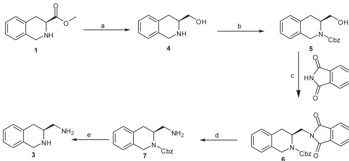
Scheme 2
