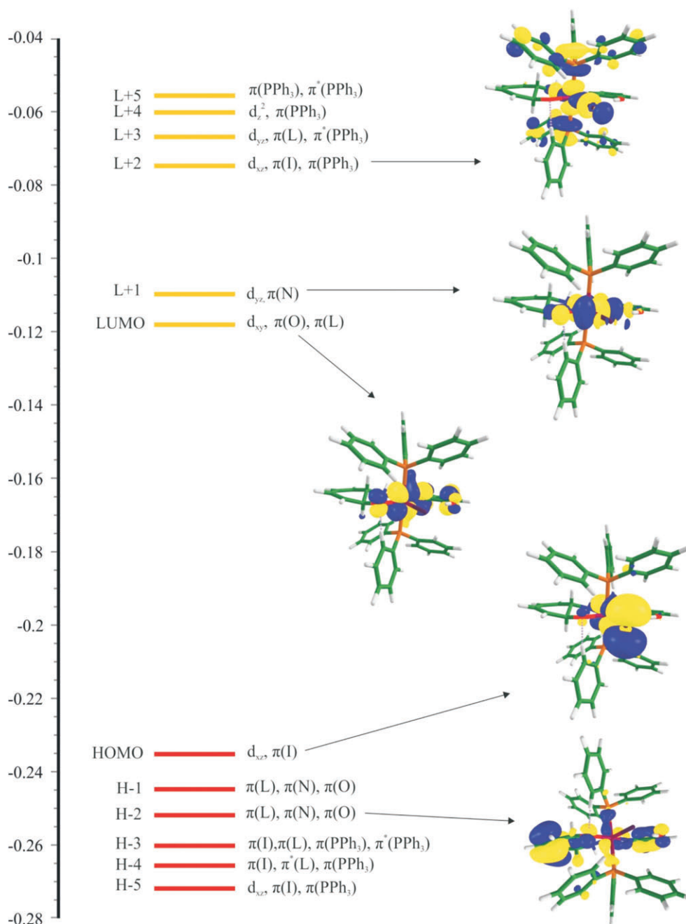
Complex 2-B3LYP MO Energy Diagram (CHCl 3 )
