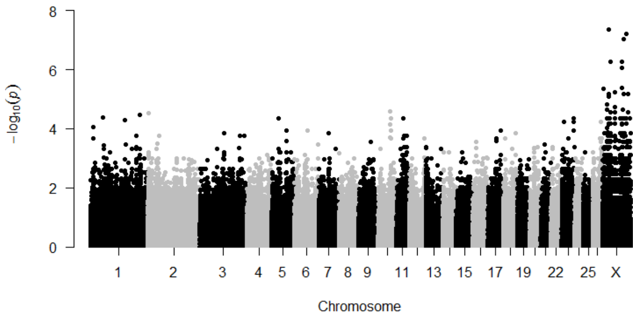
Figure 4 Manhattan plot of results from Fisher's exact test for association of SNP genotype with wet carcass syndrome based on samples from only the 38 males. The physical position of the SNP according to chromosome number is plotted on the x-axis, while the -\log_{10}P -values are plotted on the y-axis
