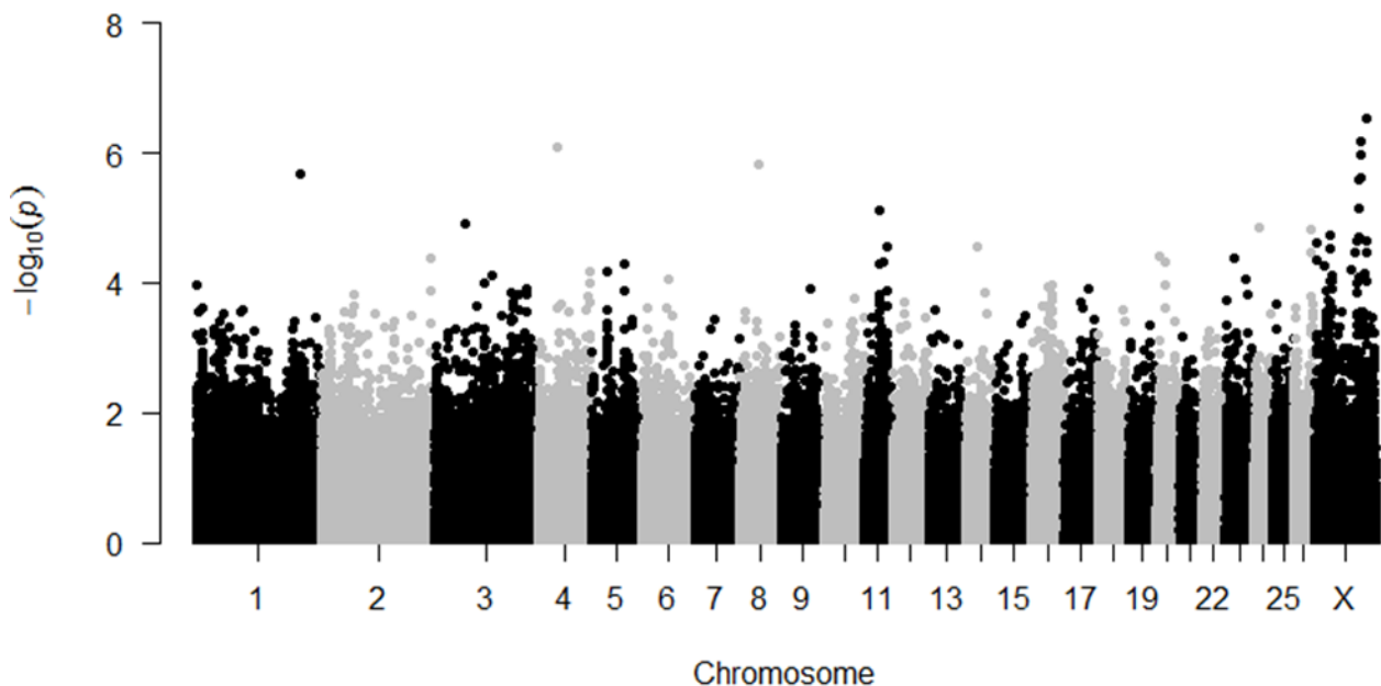
Figure 3 Manhattan plot of results from Fisher's exact for association of SNP genotype with wet carcass syndrome based on 69 samples from both males and females. The physical position of the SNP according to chromosome number is plotted on the x-axis, while the -\log_{10}P -values are plotted on the y-axis
