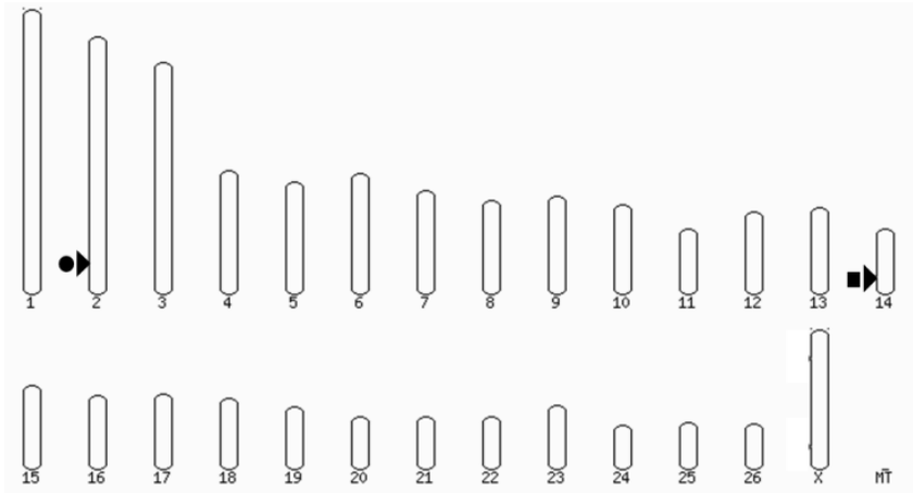
Figure 2 Position of PRKAG3 on chromosome 2 and RYR1 on chromosome 14 in the ovine genome
