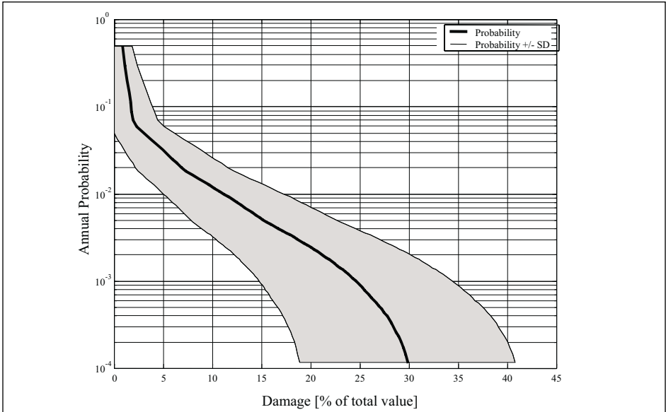
FIGURE 8. Risk curve for high-rise facilities with reinforced concrete shear walls without moment-resisting frames
