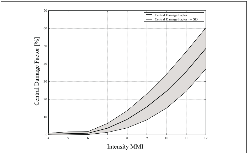
FIGURE 4. Vulnerability curve for low rise facilities with reinforced concrete shear walls, without moment-resisting frames
