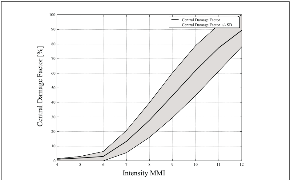
FIGURE 3. Vulnerability curve for medium rise facilities with reinforced concrete shear walls and moment-resisting frames
