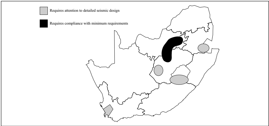
FIGURE 5. SABS areas requiring adherence to specific seismic building requirements
