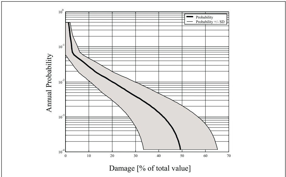
FIGURE 7. Risk curve for medium-rise facilities with reinforced concrete shear walls without moment-resisting frames
