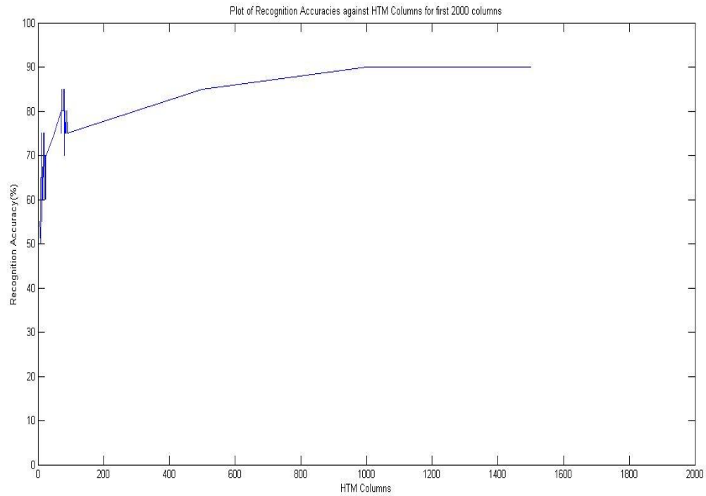
Figure 4: Graphical representation of test results for the HTM/CLA system
