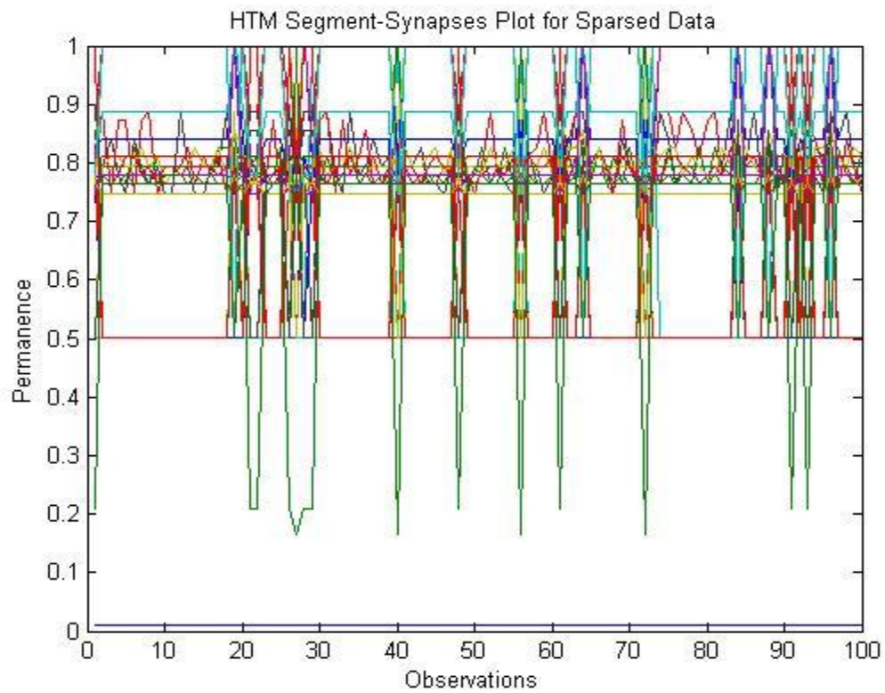
Figure 6: Visualization of Sparse HTM Segment Synapses of CCF data after Training
