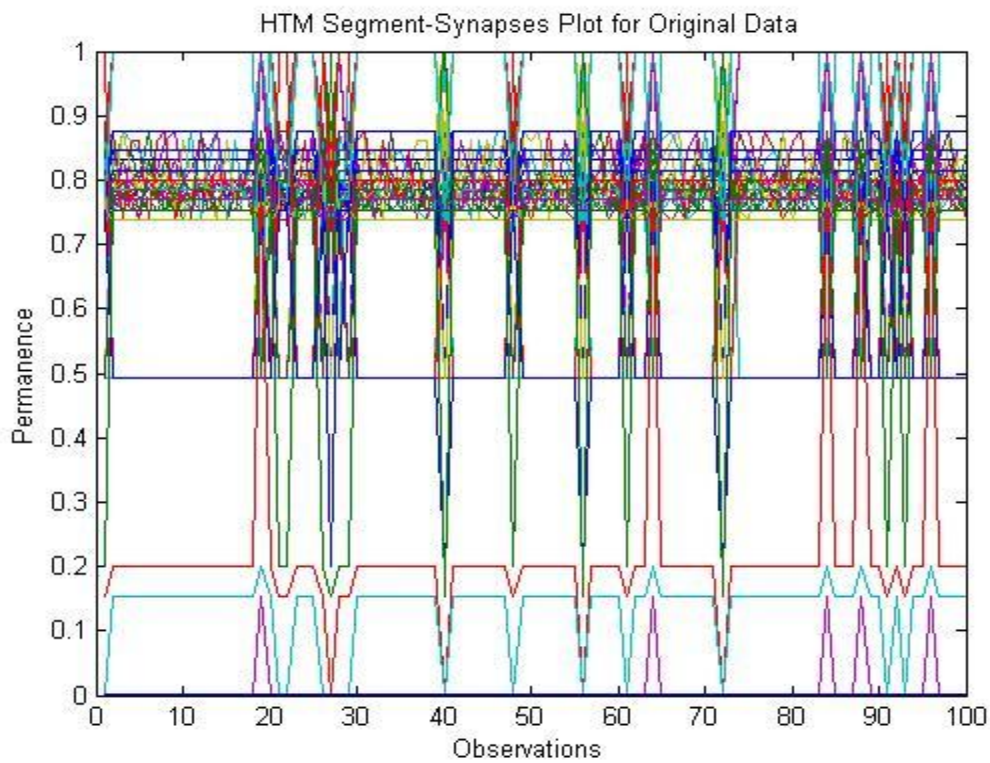
Figure 5: Visualization of HTM Segment Synapses of CCF data for Training
